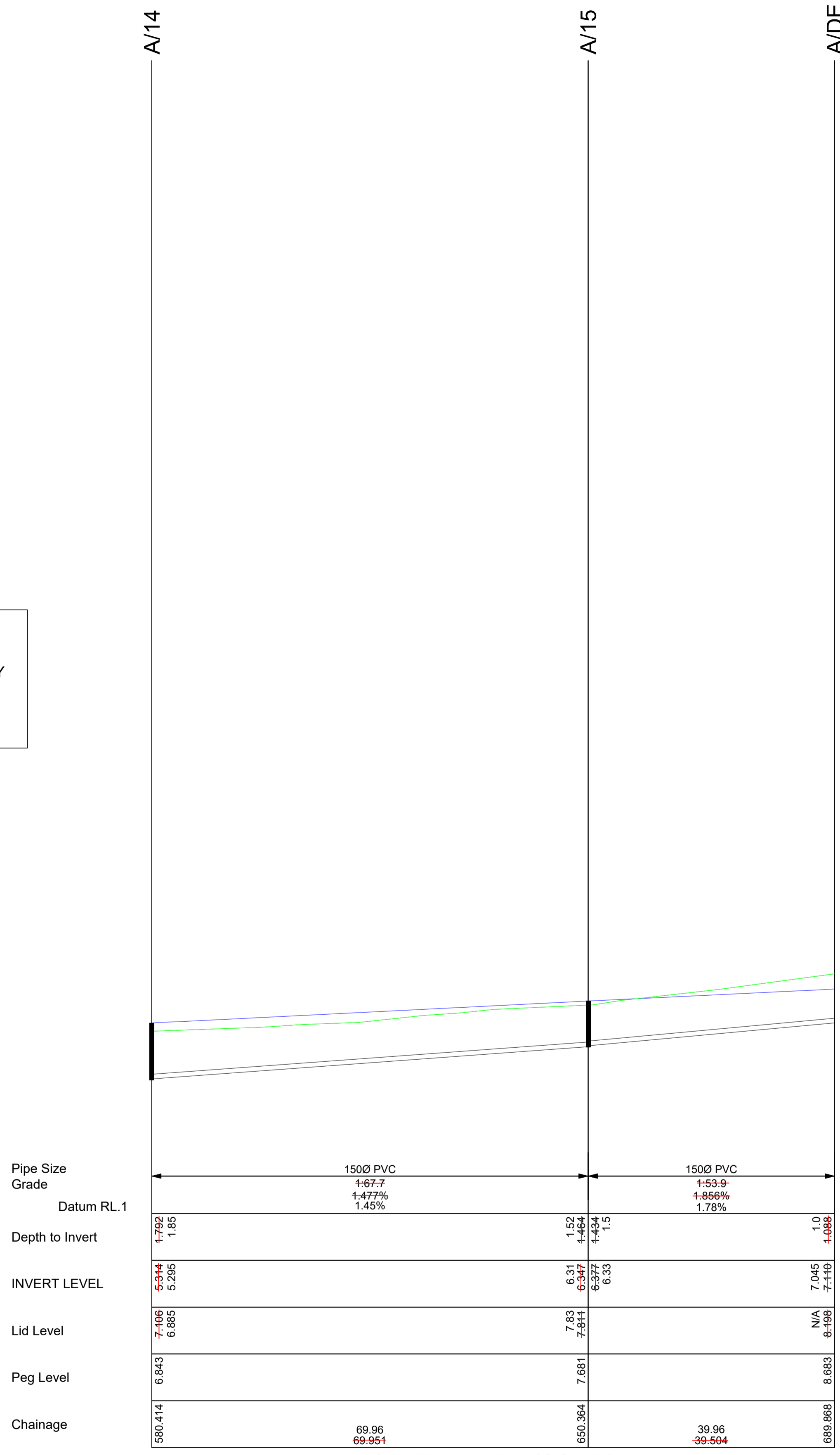
SEWER LINE A (CONT.) SCALES: HORIZONTAL 1:500 VERTICAL 1:100
