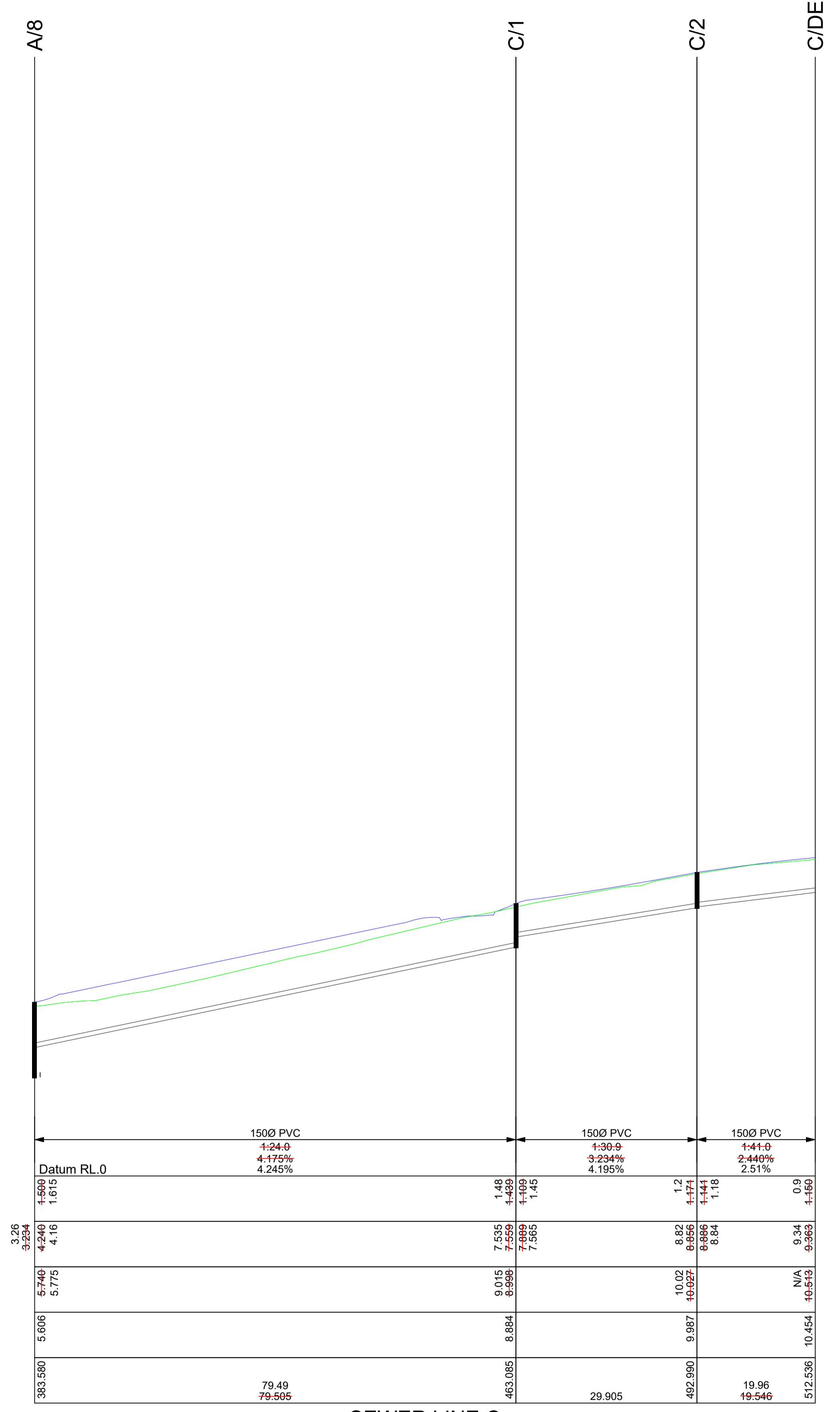
SEWER LINE C SCALES: HORIZONTAL 1:500 VERTICAL 1:100
