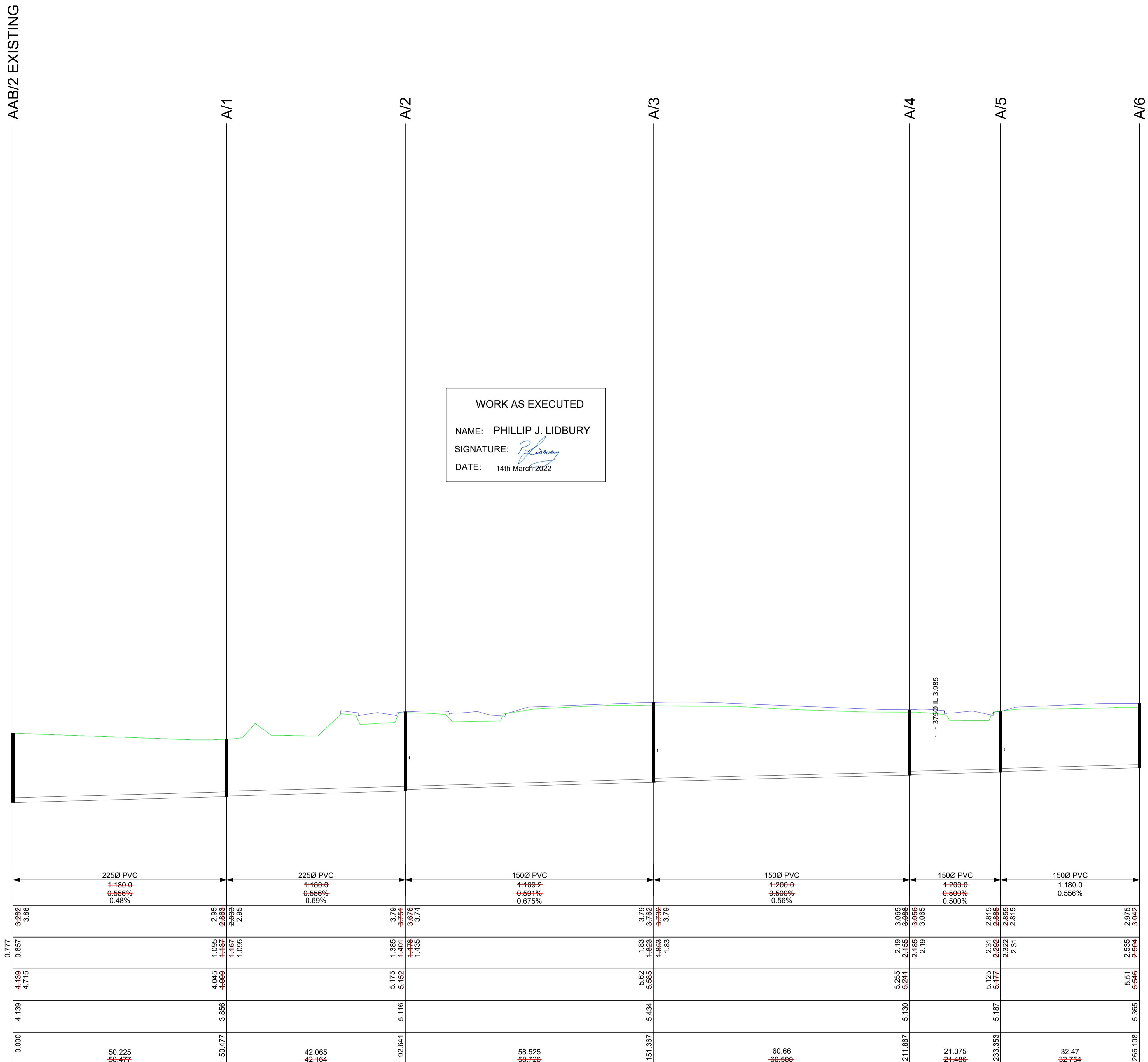
SEWER LINE A SCALES: HORIZONTAL 1:500 VERTICAL 1:100
