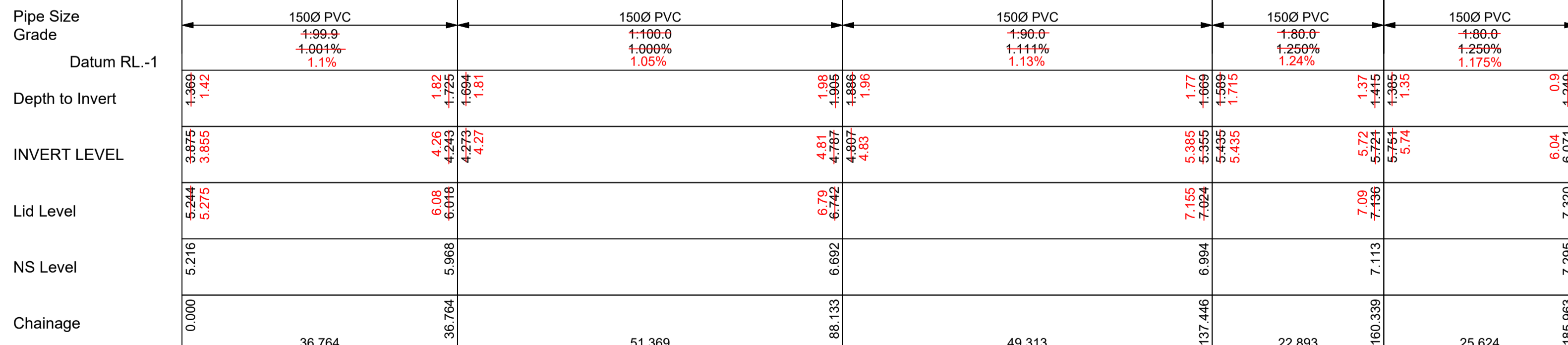
SEWER LINE K SCALES: HORIZONTAL 1:500 VERTICAL 1:100
