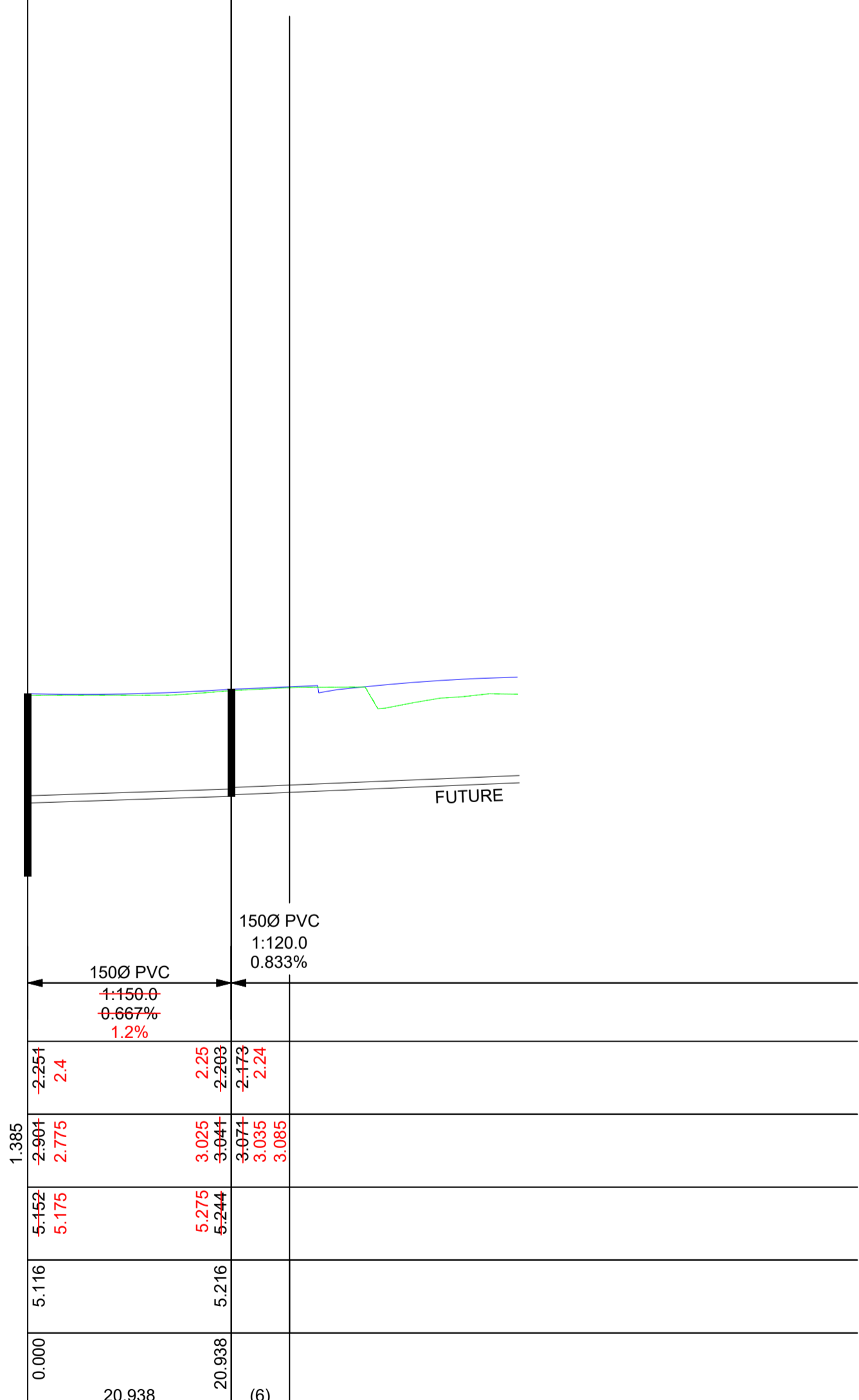
SEWER LINE J SCALES: HORIZONTAL 1:500 VERTICAL 1:100
